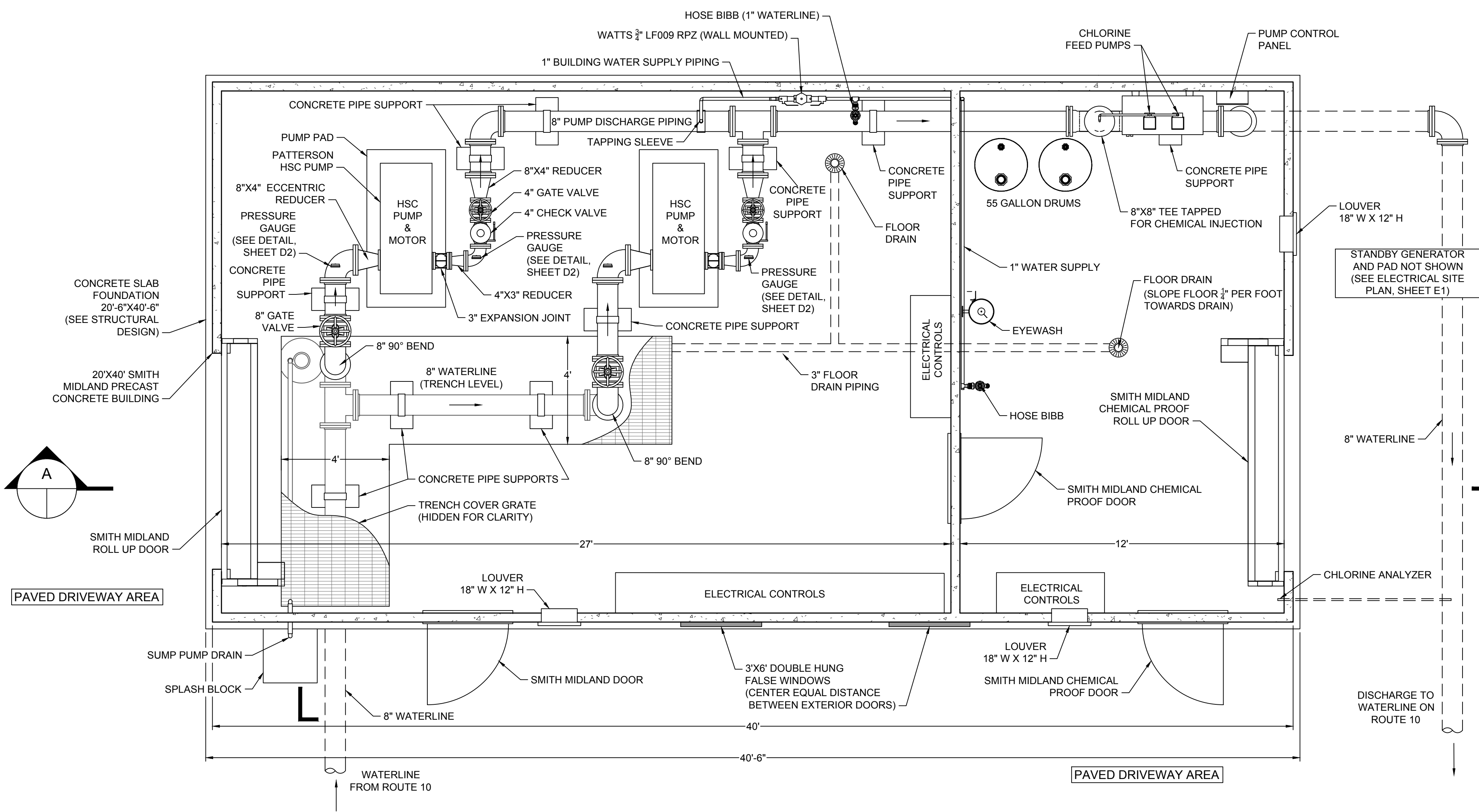
BOOSTER PUMP STATION FLOOR PLAN
