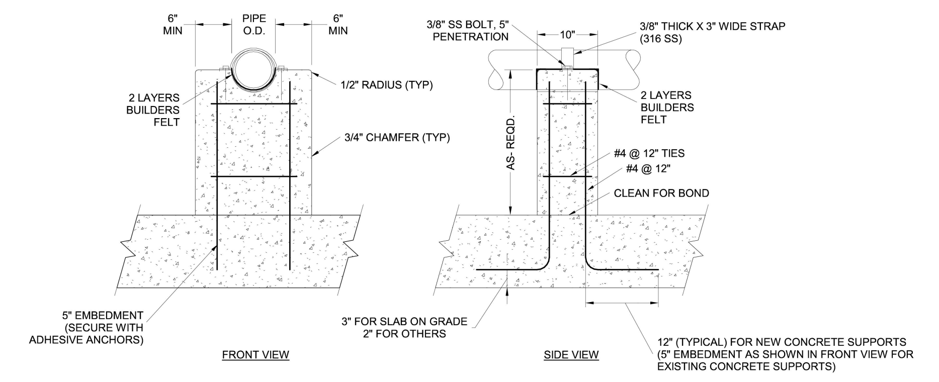
CONCRETE PIPE SUPPORT DETAIL
